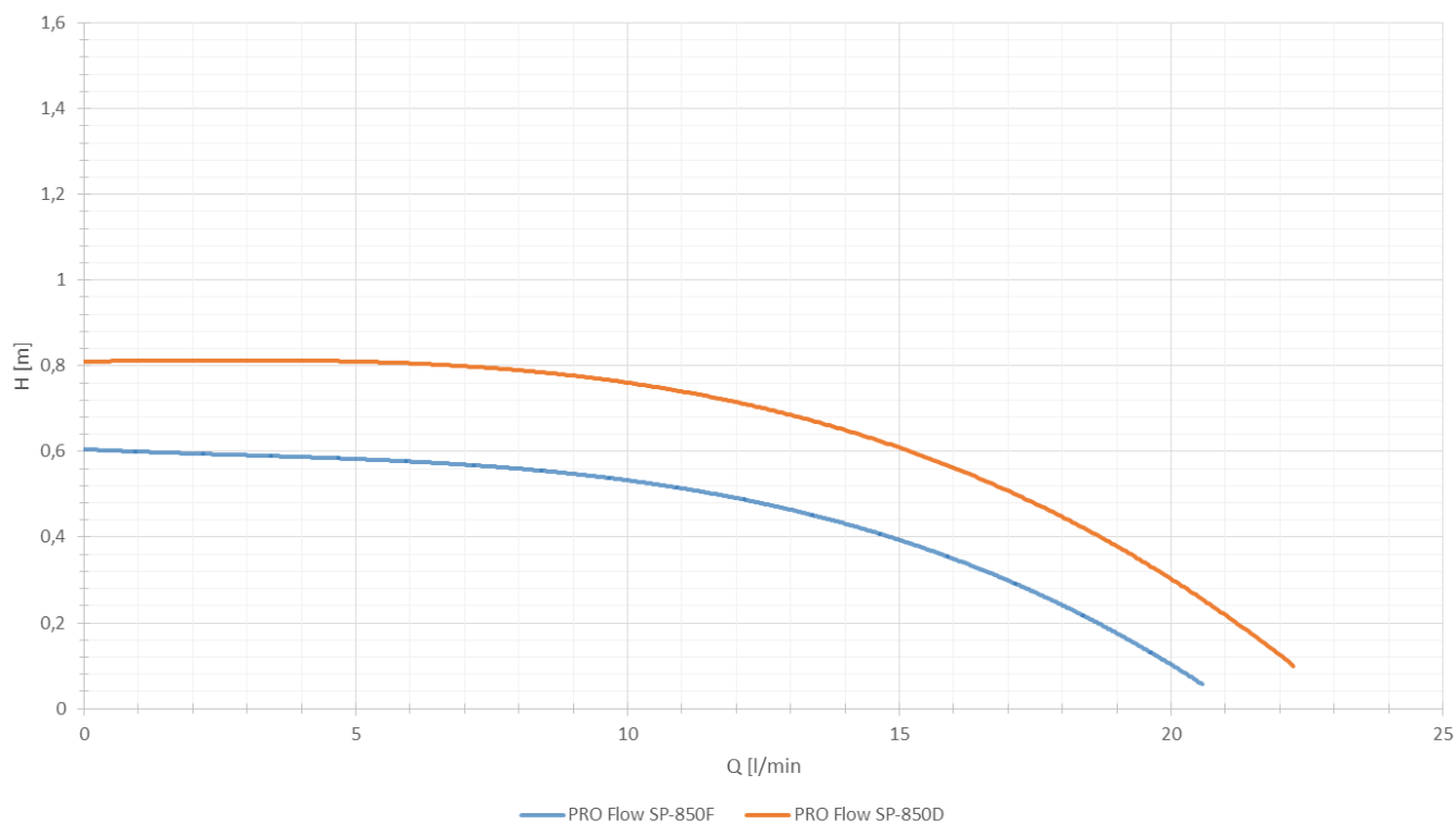
PRO Flow SP-850D vs PRO Flow SP 850F, 600 U/min
