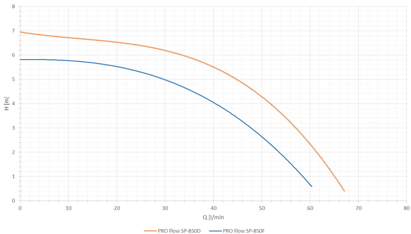
PRO Flow SP-850D vs PRO Flow SP 850F, 1800 U/min
