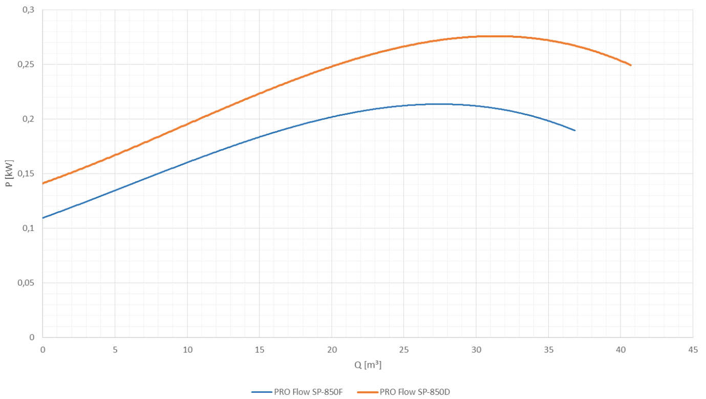
PRO Flow SP-850D vs PRO Flow SP 850F, 1100 U/min
