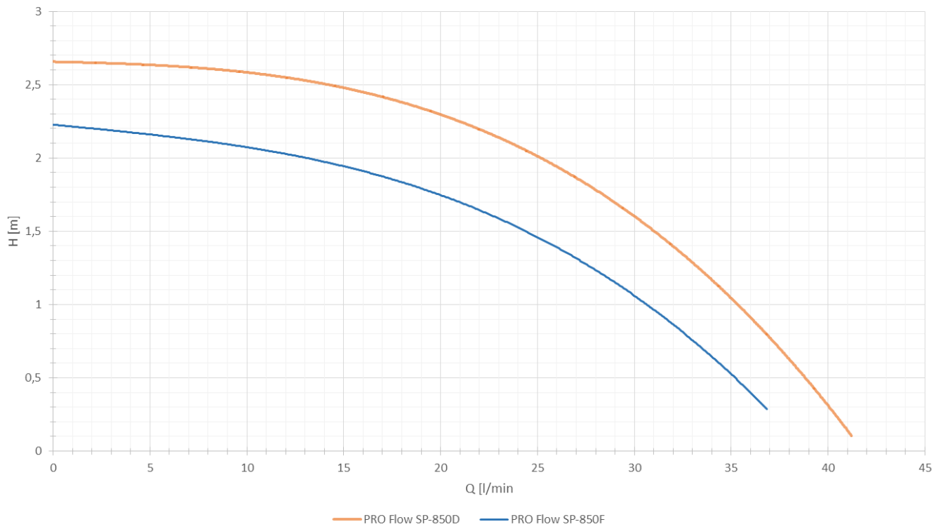
PRO Flow SP-850D vs PRO Flow SP 850F, 1100 U/min
